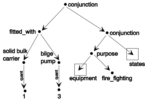
Figure 4: Network underlying (11)
